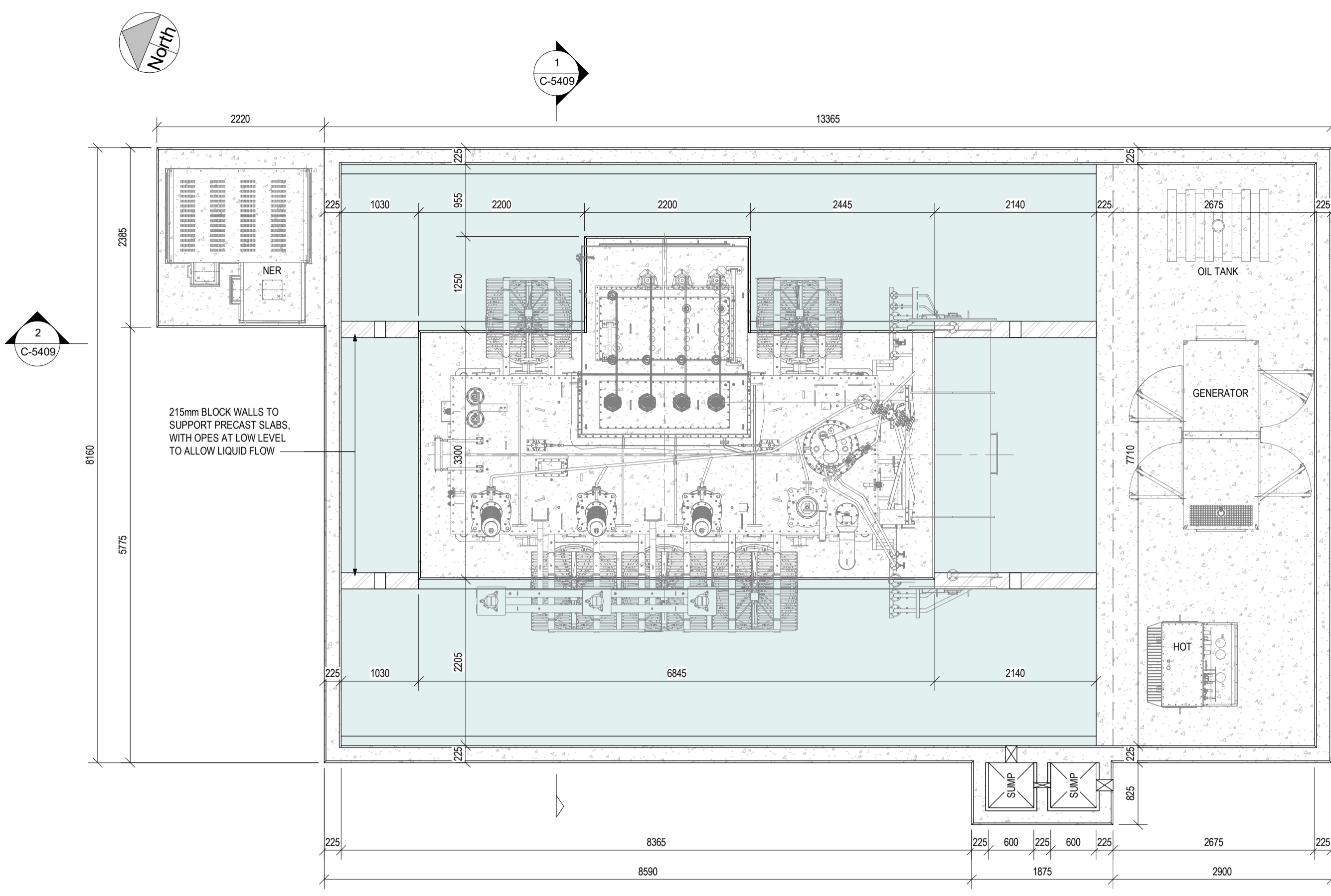
TRANSFORMER BUND & PLINTH SCALE 1 : 50
