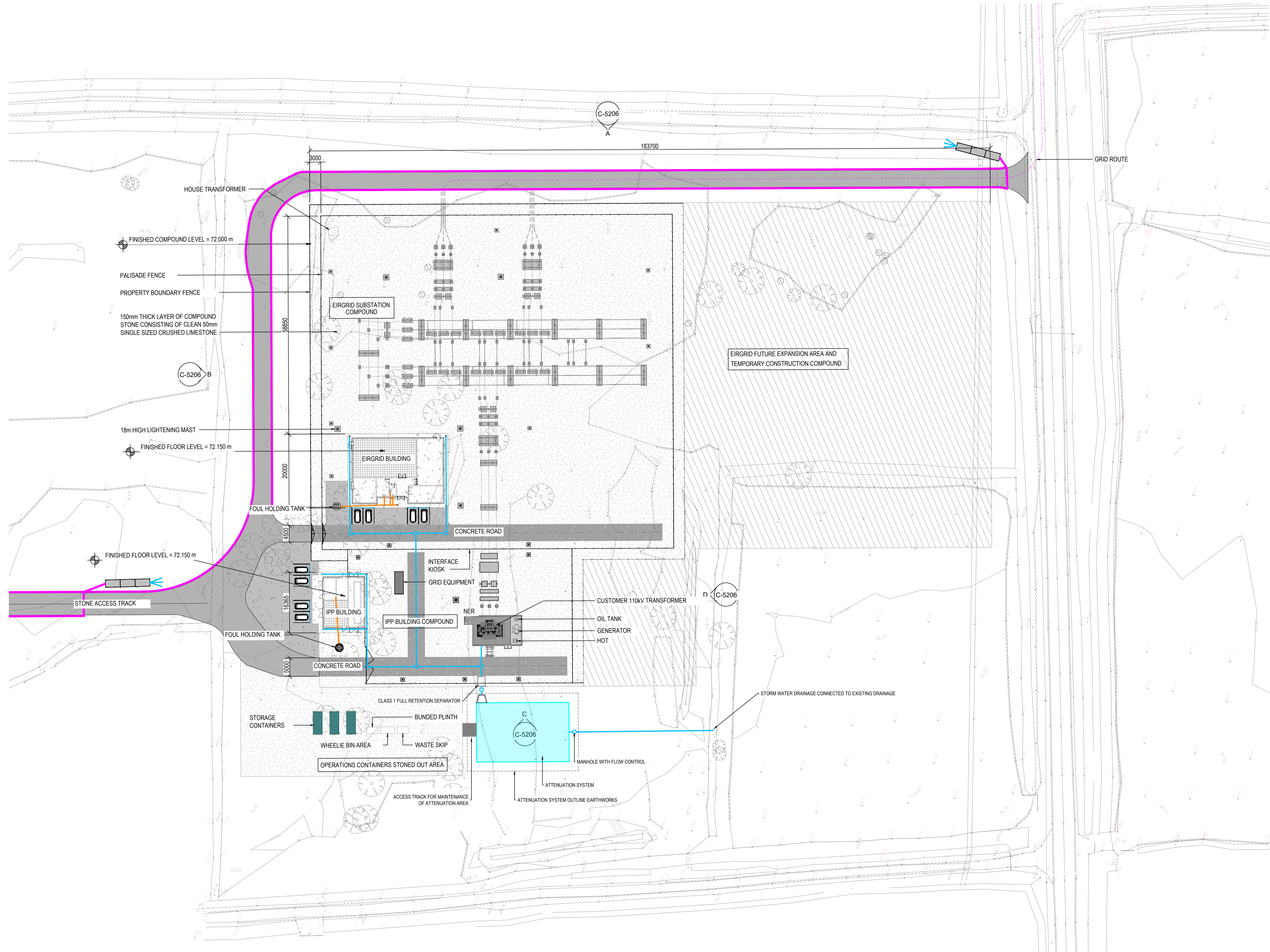
SUBSTATION DRAINAGE & WATER SERVICE LAYOUT SCALE 1 : 500
