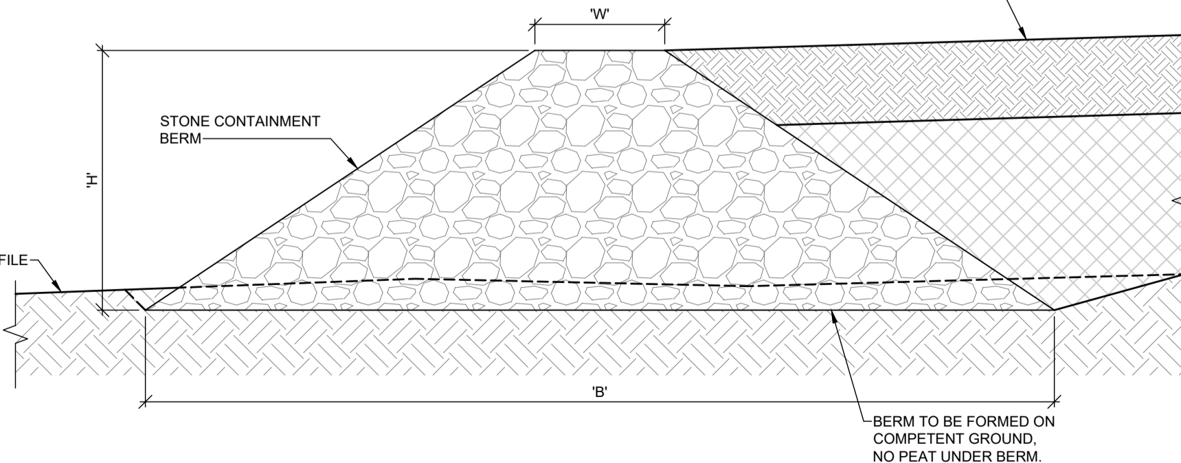
SPOIL STORAGE CONTAINMENT BERM DETAIL SCALE 1:20
