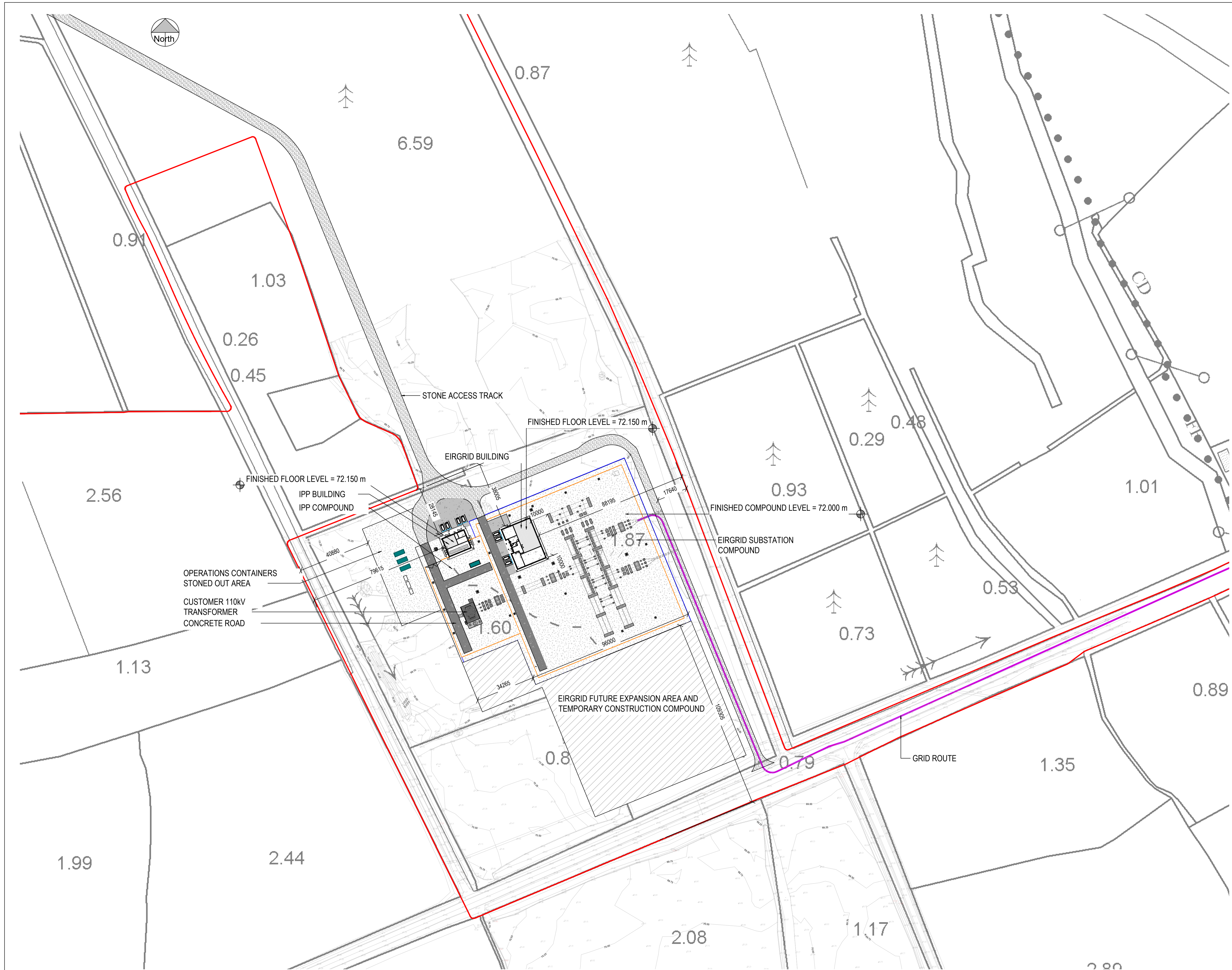
WF SUBSTATION SITE LAYOUT SCALE 1: 1000
